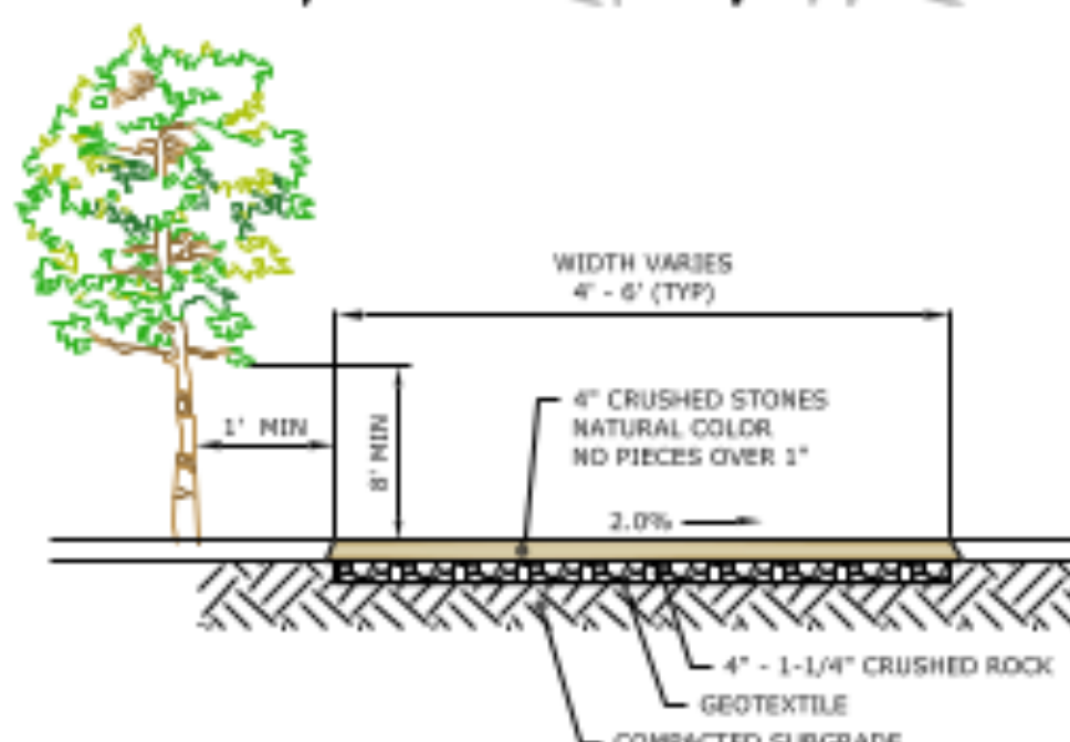
CROSS COUNTRY TRACK SECTION N.T.S.
